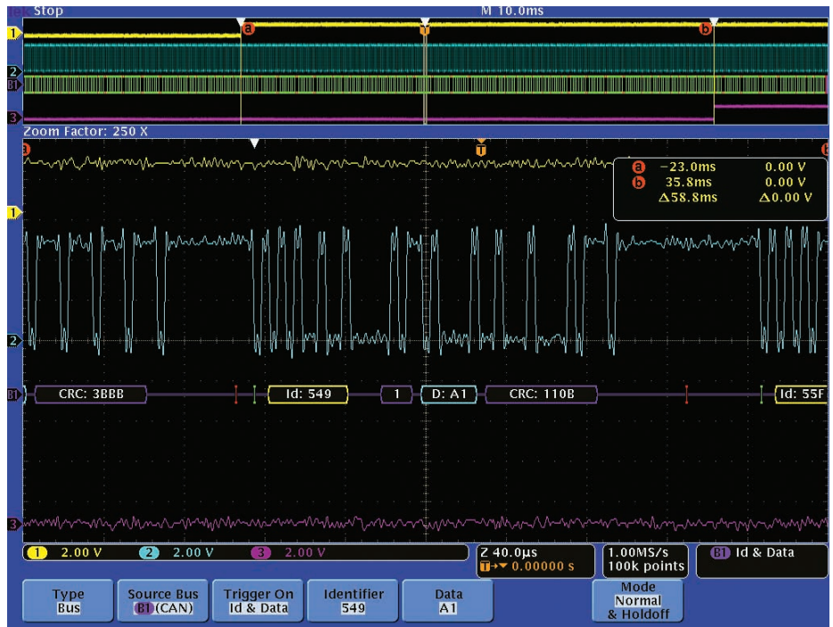
Figure 28. Triggering on specific identifier and Data on a CAN bus and decoding all messages in the acquisition.
