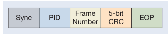
Figure 21. Start of frame packets.
