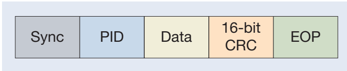
Figure 20. Data Packets with the PID of DATA0 or DATA1.
