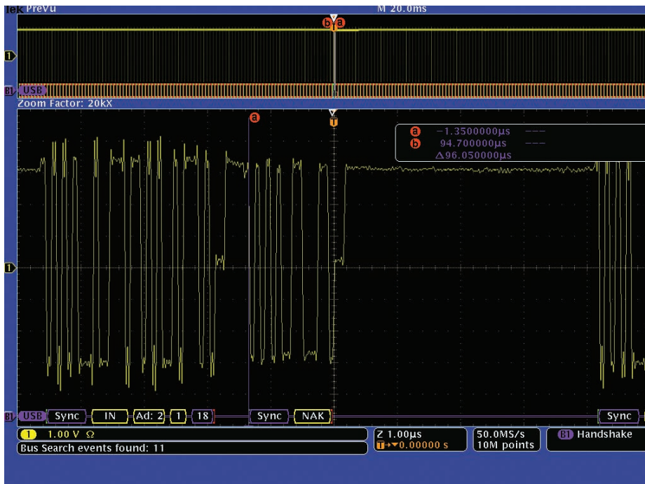
Figure 22. Full-speed memory device responded with a NAK to the host first IN token request at cursor A.
