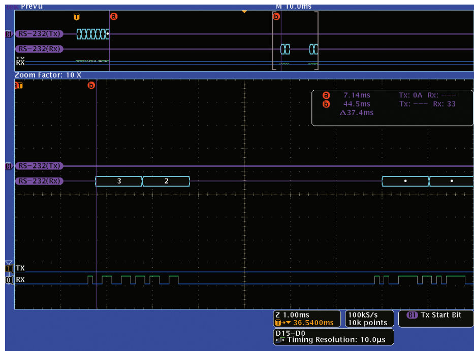
Figure 25. Measuring time delay between messages on two RS-232 buses.
