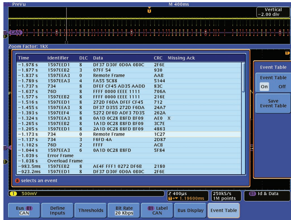
Figure 29. CAN event table.
