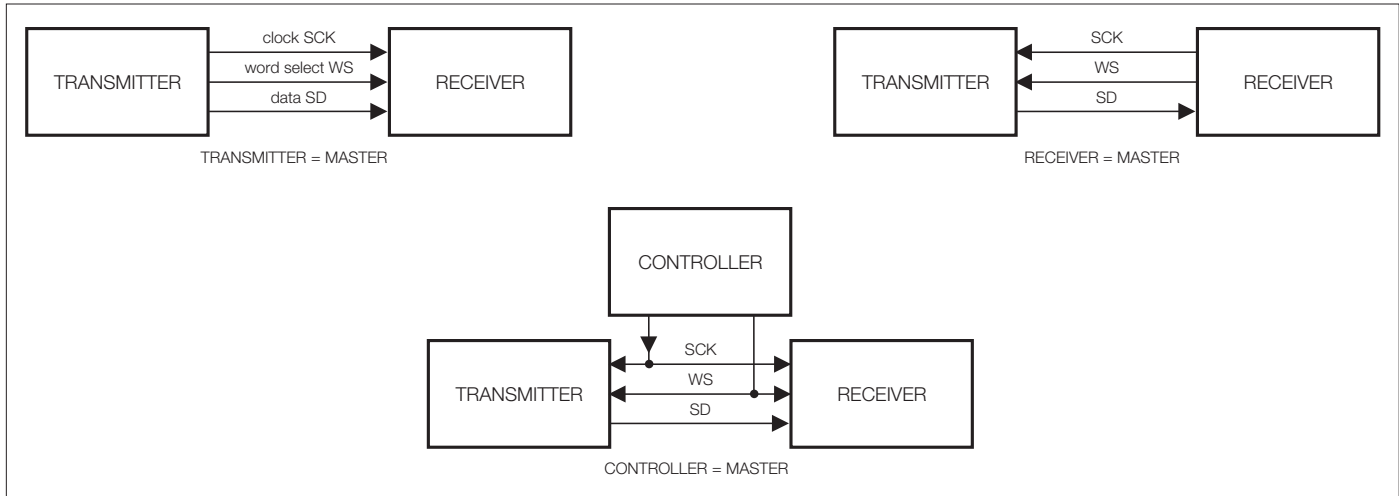
Figure 38. Different I²S bus configurations.
