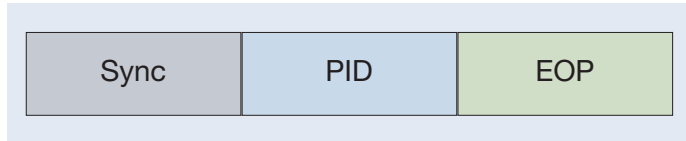
Figure 18. Handshake packet organization.
