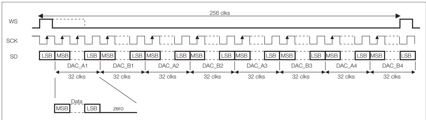
Figure 40. TDM Format.
