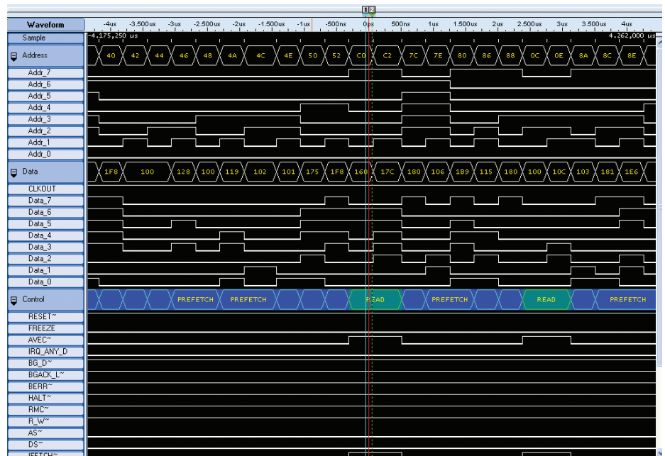
Figure 1. Logic Analyzer acquisition of a microcontroller's clock, address bus, data bus and control lines.
