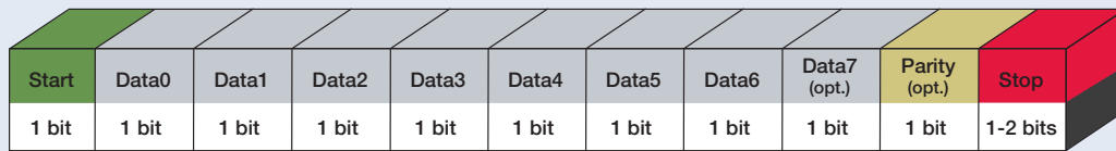
Figure 23. RS-232 byte structure.
