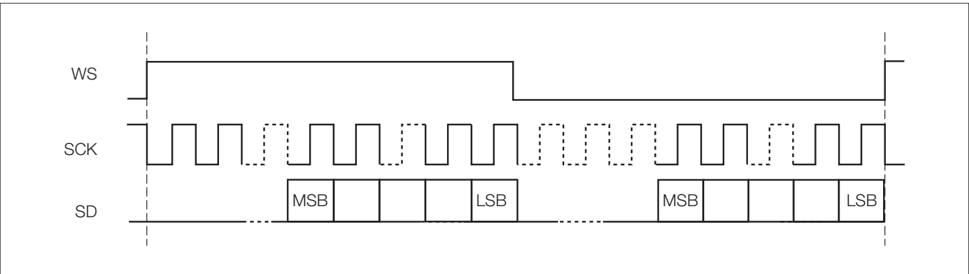
Figure 39 part III. RJ Format.
