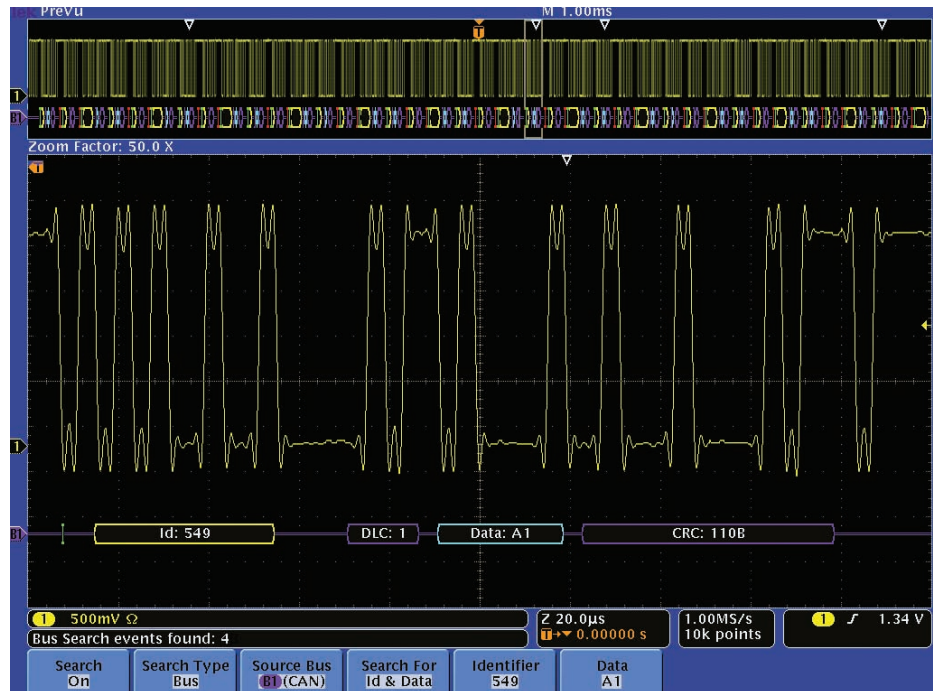
Figure 37. Searching on specified identifier and Data in a CAN bus acquisition.
