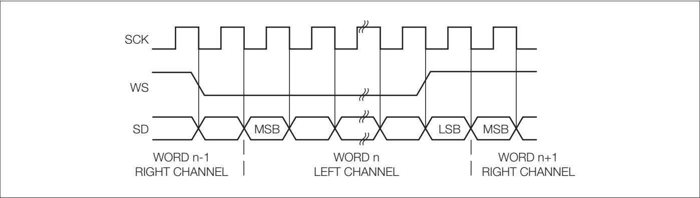
Figure 39 part I. I²S Format.
