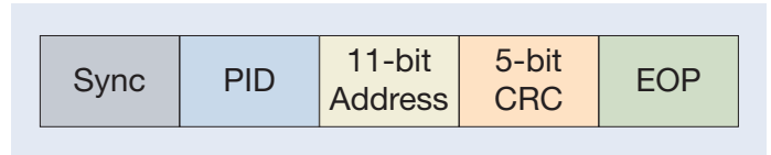
Figure 19. OUT, IN and SETUP token packet organization.
