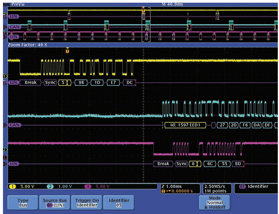
Figure 32. Simultaneous capture and decode of multiple automotive serial buses.
