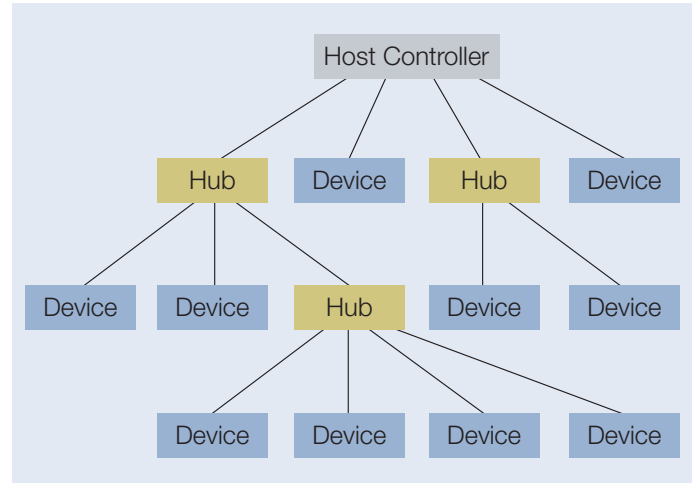
Figure 14. USB tiered-star topology uses hubs to expand the bus.
