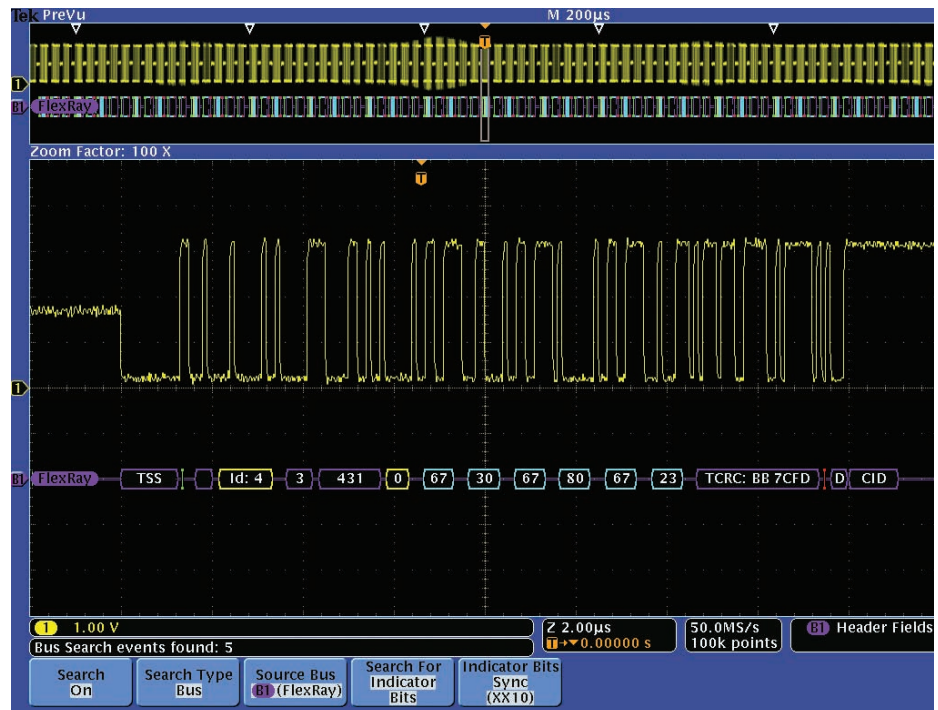
Figure 35. Triggering on Frame ID and Cycle Count, Searching through acquired data for Startup Frames.
